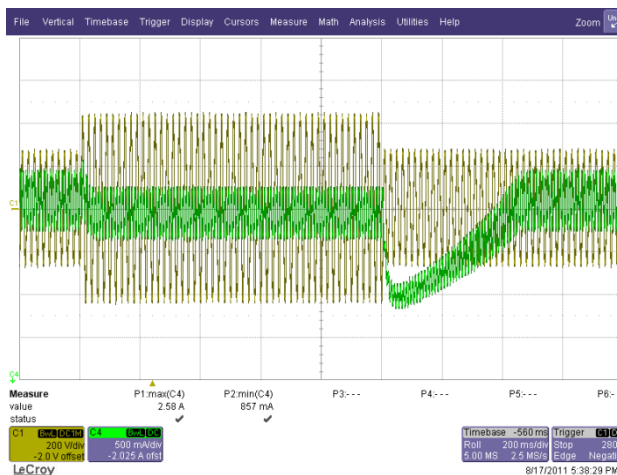
Figure 32 – 180-300-180 VAC / 50 Hz, 1 s Pulse. Load: 32 V LED String. Ch1: V_{IN} , 200 V / div. Ch4: I_{OUT} , 500 mA / div., 200 ms / div.
