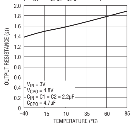
2x Mode Charge Pump Open-Loop Output Resistance ( 2V_{IN} - V_{CPO} )/ I_{CPO} vs Temperature
