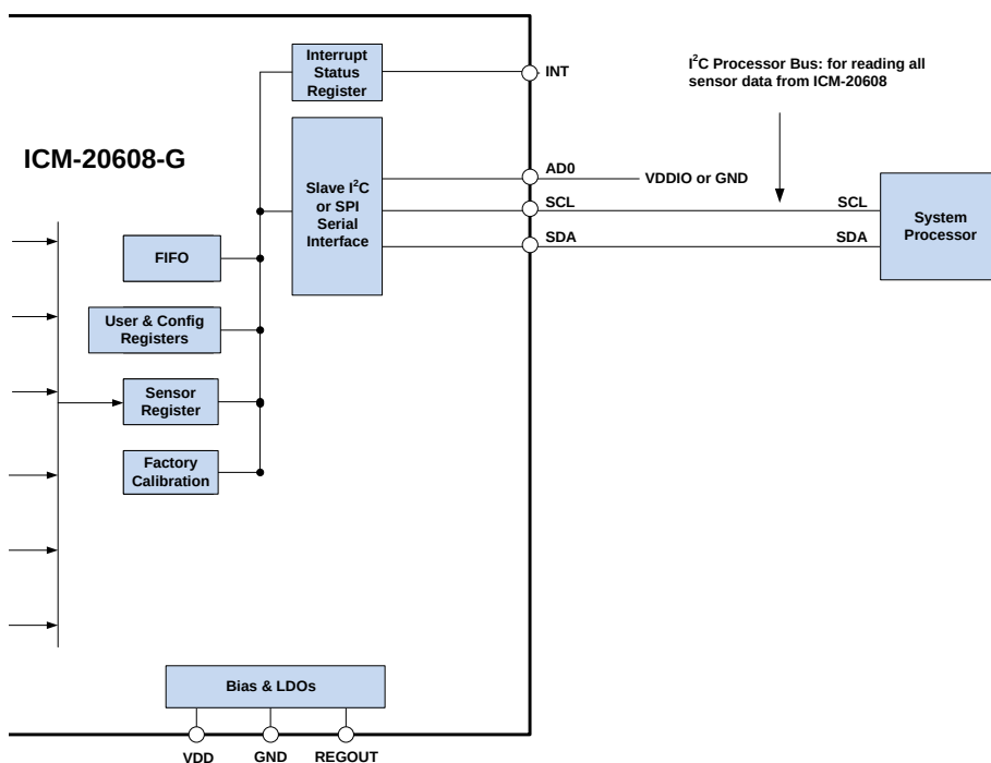
Figure 7. ICM-20608-G Solution Using I²C Interface
