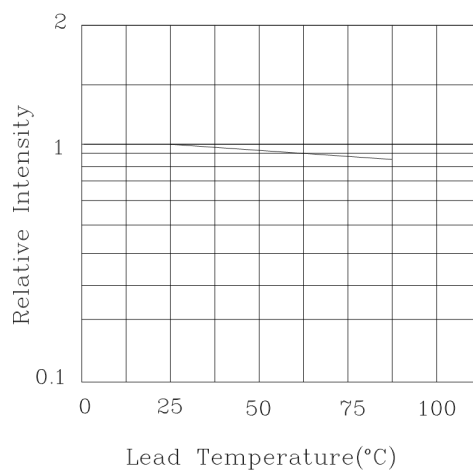
RELATIVE INTENSITY VS. LEAD TEMPERATURE
