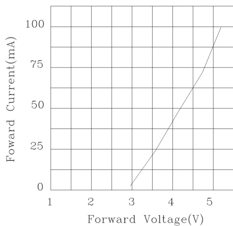
PEAK FORWARD VOLTAGE VS. FORWARD CURRENT
