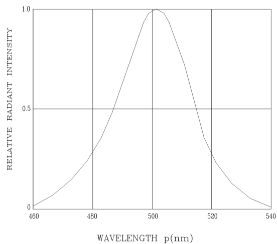
SPECTRAL DISTRIBUTION
