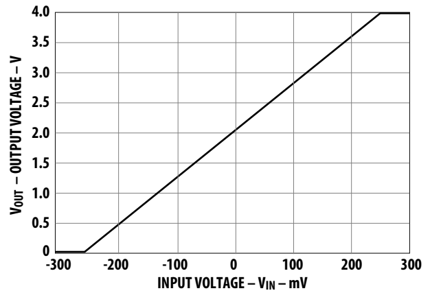
Figure 6. V_{OUT} vs. V_{IN} .
