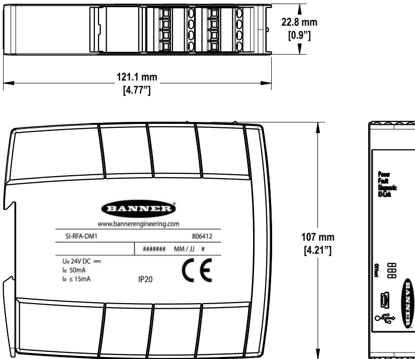
Figure 5. SI-RF-DM1 Module
