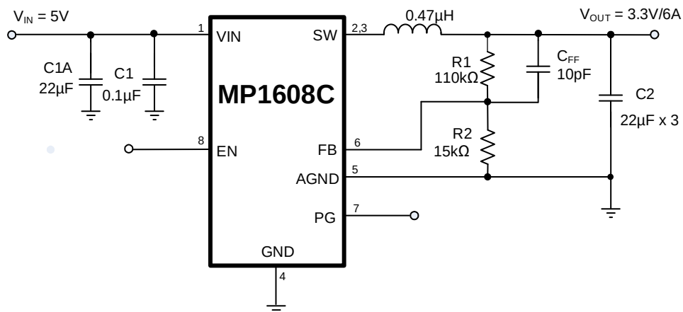
Figure 9: Typical Application Circuit ( V_{IN} = 5V , V_{OUT} = 3.3V/6A )
