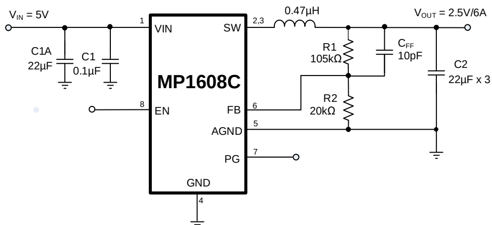
Figure 8: Typical Application Circuit ( V_{IN} = 5V , V_{OUT} = 2.5V/6A )
