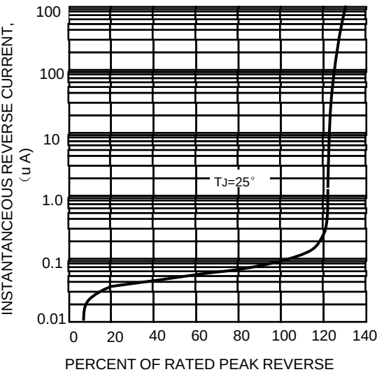
FIG.3-TYPICAL REVERSE CHARACTERISTICS
