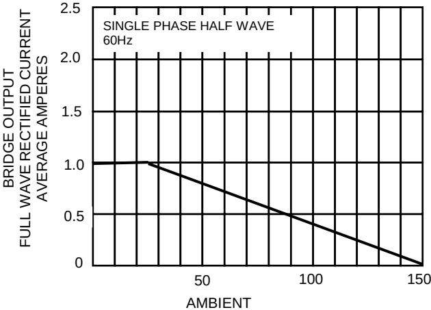
FIG.1-DERATING CURVE FOR
