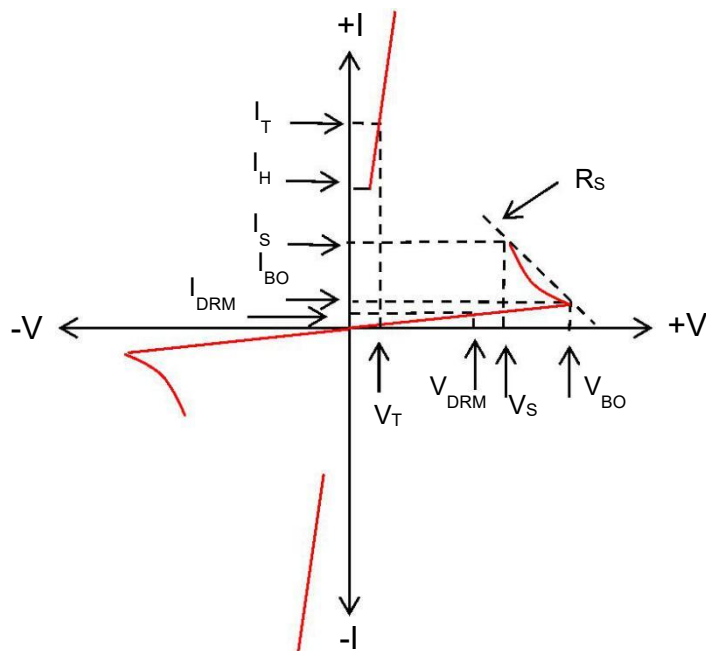
Figure 1. V-I Characteristics
