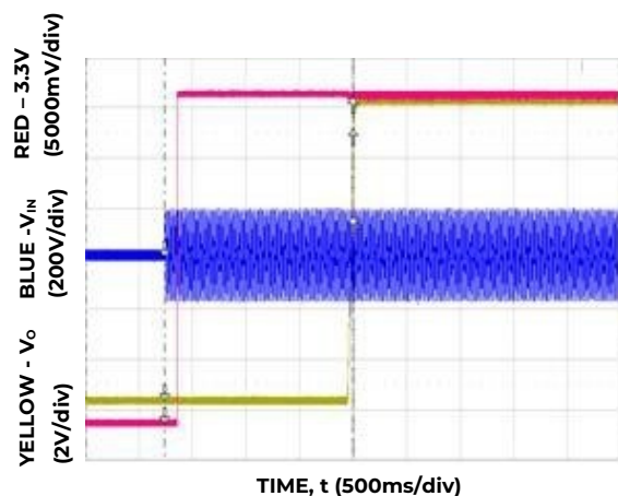
Figure 5. Typical Start-up ( V_{IN} = 230V_{ac} ).
