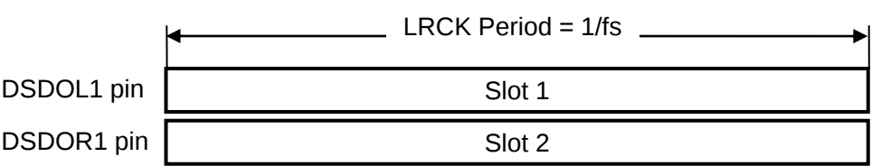
Figure 58. Slot Assign in DSD mode
