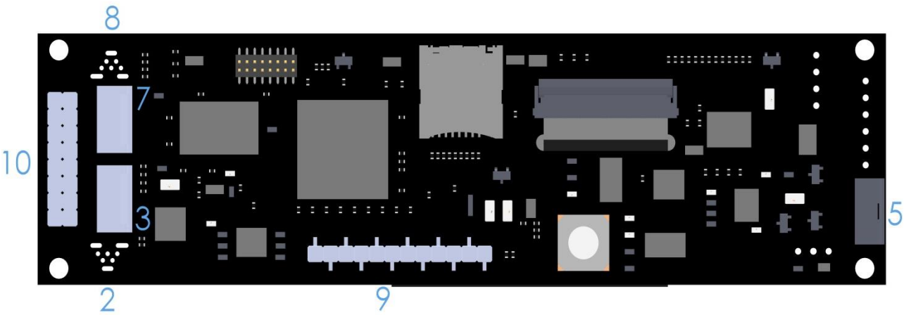
Figure 9: GTT38A-CU Header Locations
