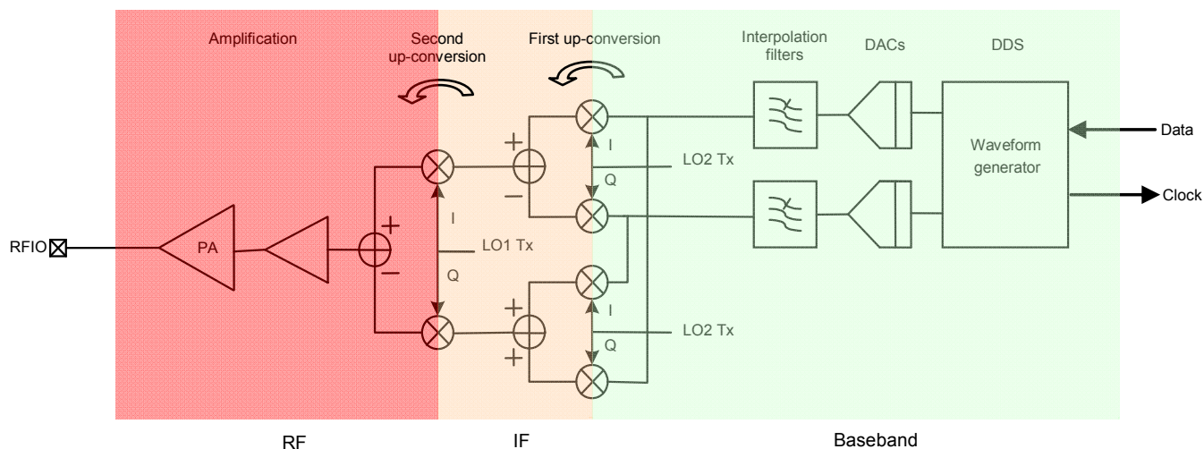
Figure 8: Transmitter Architecture
