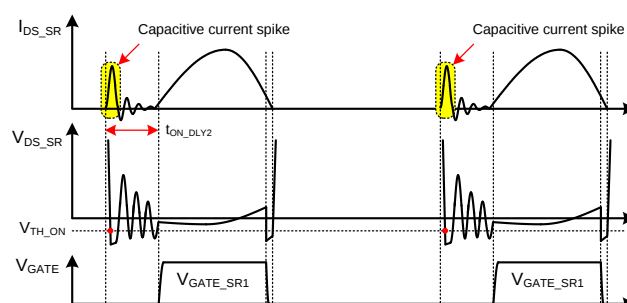
Figure 22. Capacitive current spike at light load condition
