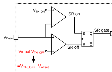
Figure 18. Virtual V_{TH\_OFF}
