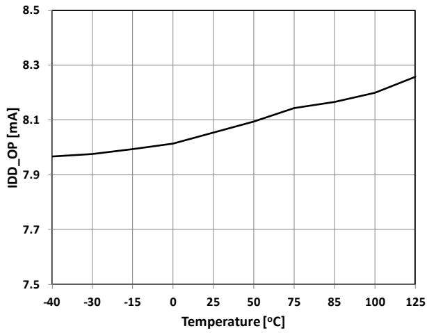
Figure 5. I DD_OP
