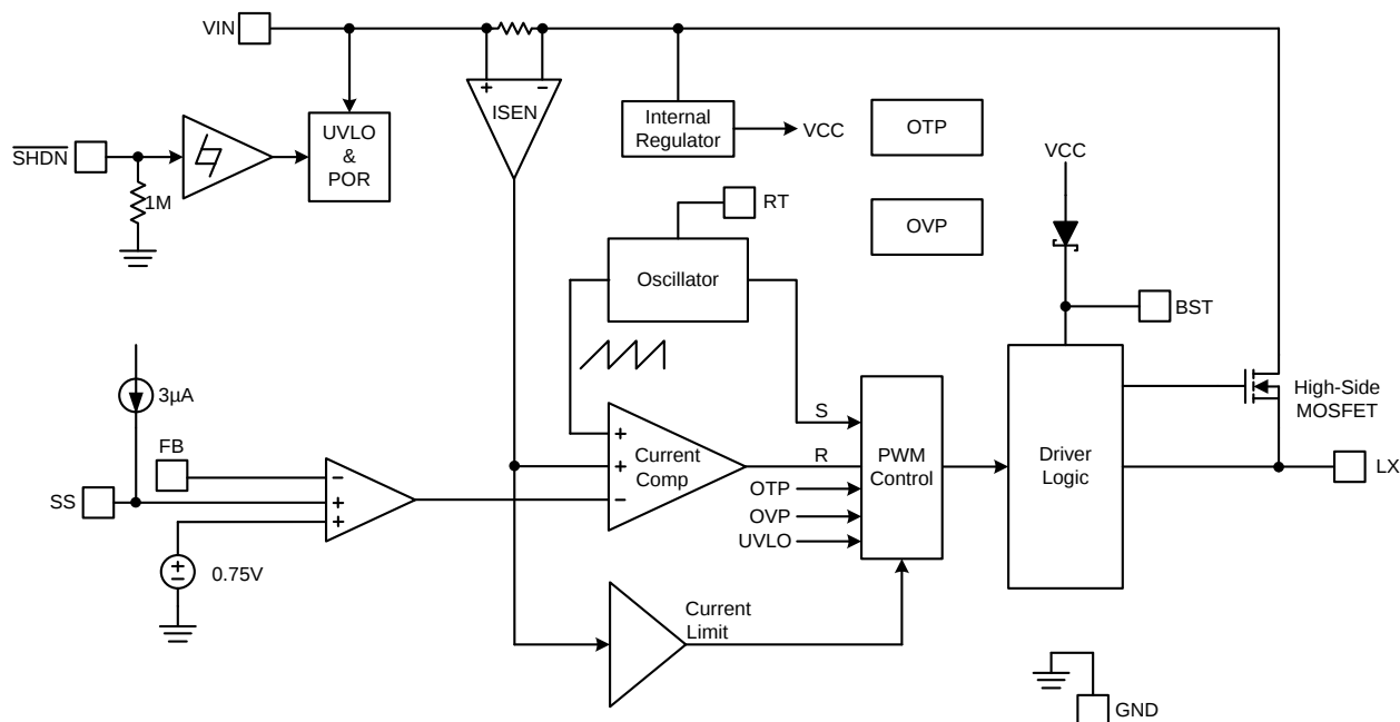
Figure 4. Block Diagram of FR9835A
