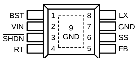
Figure 1. Pin Assignment of FR9835A
