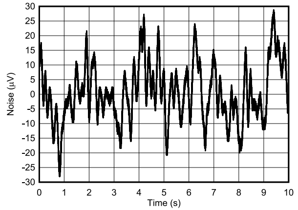
图 6-46. Digipot Output Noise: 0.1 Hz to 10 Hz
