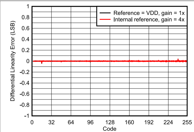
图 6-12. Differential Linearity Error vs Digital Input Code
