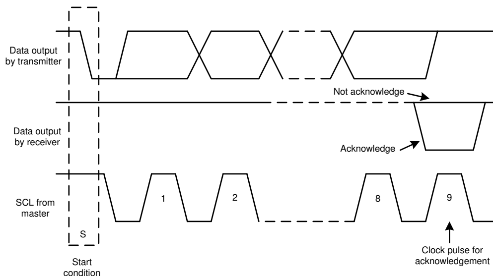
图 7-2. Acknowledge and Not Acknowledge on the I 2 C Bus
