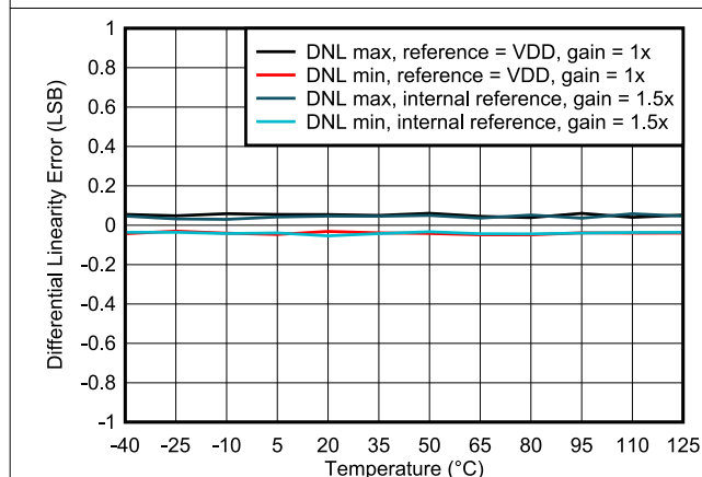
图 6-5. Differential Linearity Error vs Temperature
