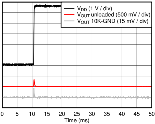
图 6-39. Power-on Glitch
