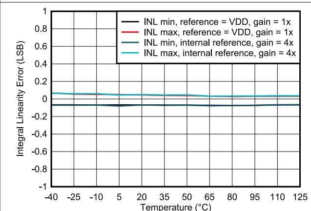
图 6-14. Integral Linearity Error vs Temperature
