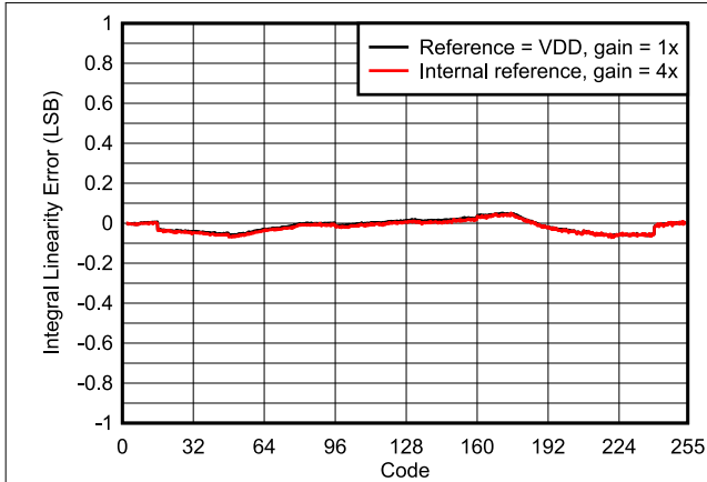
图 6-11. Integral Linearity Error vs Digital Input Code
