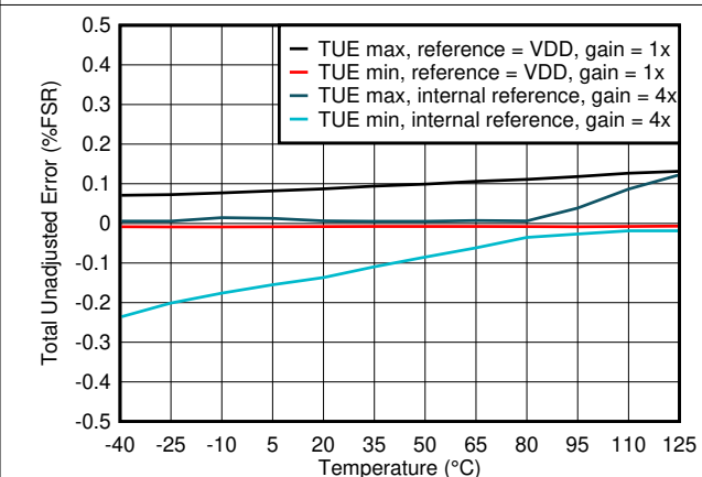
图 6-16. Total Unadjusted Error vs Temperature
