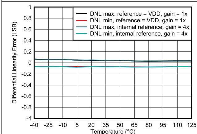
图 6-15. Differential Linearity Error vs Temperature
