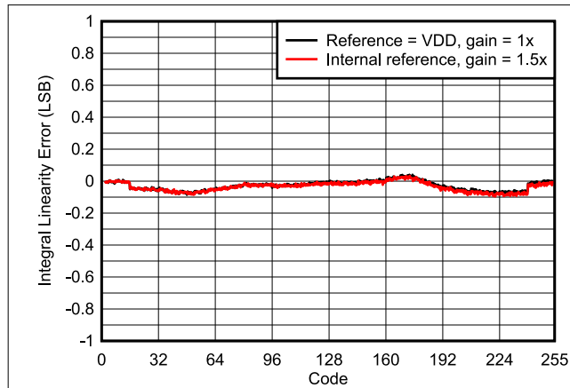
图 6-1. Integral Linearity Error vs Digital Input Code
