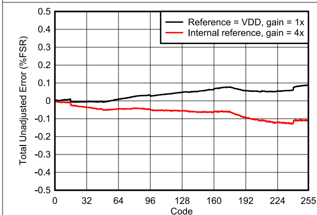
图 6-13. Total Unadjusted Error vs Digital Input Code
