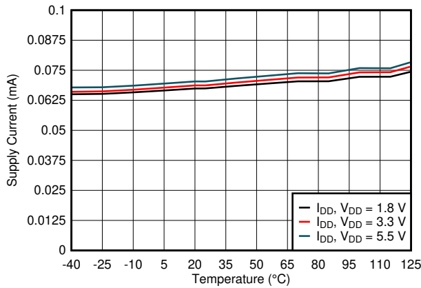
图 6-33. Power-Down Current vs Temperature
