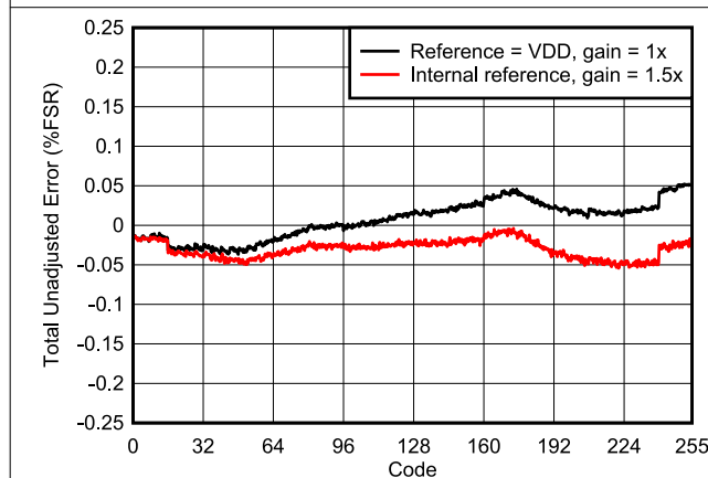
图 6-3. Total Unadjusted Error vs Digital Input Code
