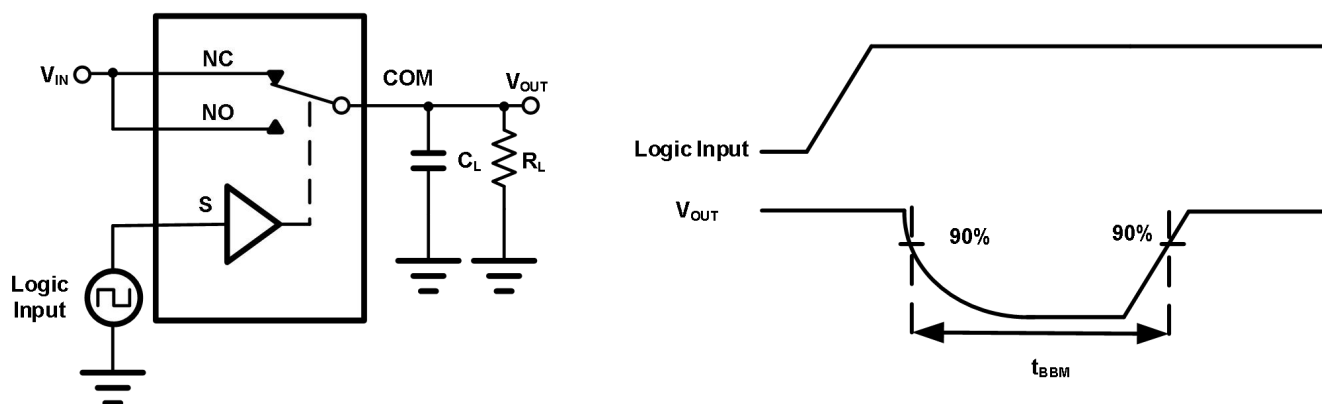
Fig.9-3. Break-Before-Make Time( t_{BBM} )
