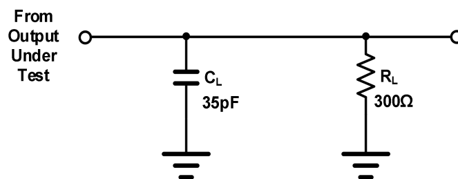
Fig.9-1. AC Test Circuit
