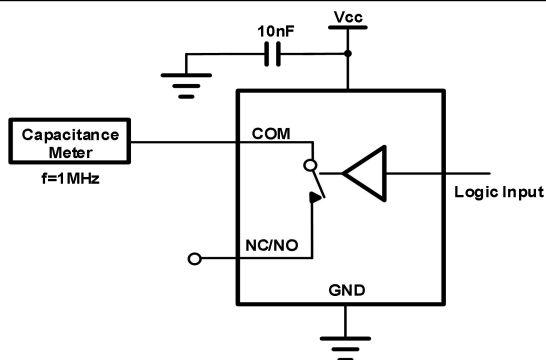
Fig.9-8. Channel On Capacitance
