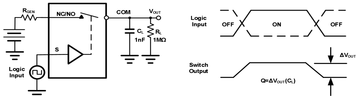
Fig.9-4. Charge Injection Test
