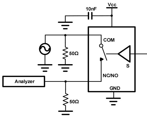
Fig.9-5. OFF Isolation ( O_{iso} )
