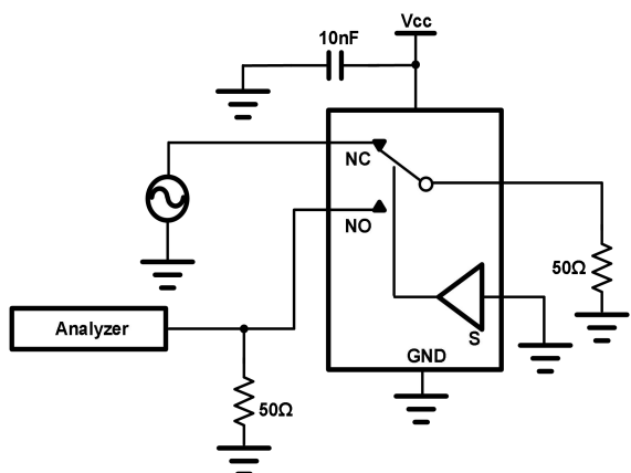
Fig.9-6. Crosstalk( X_{TALK} )
