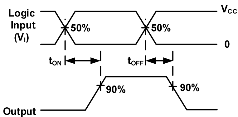
Fig.9-2. Switching Time
