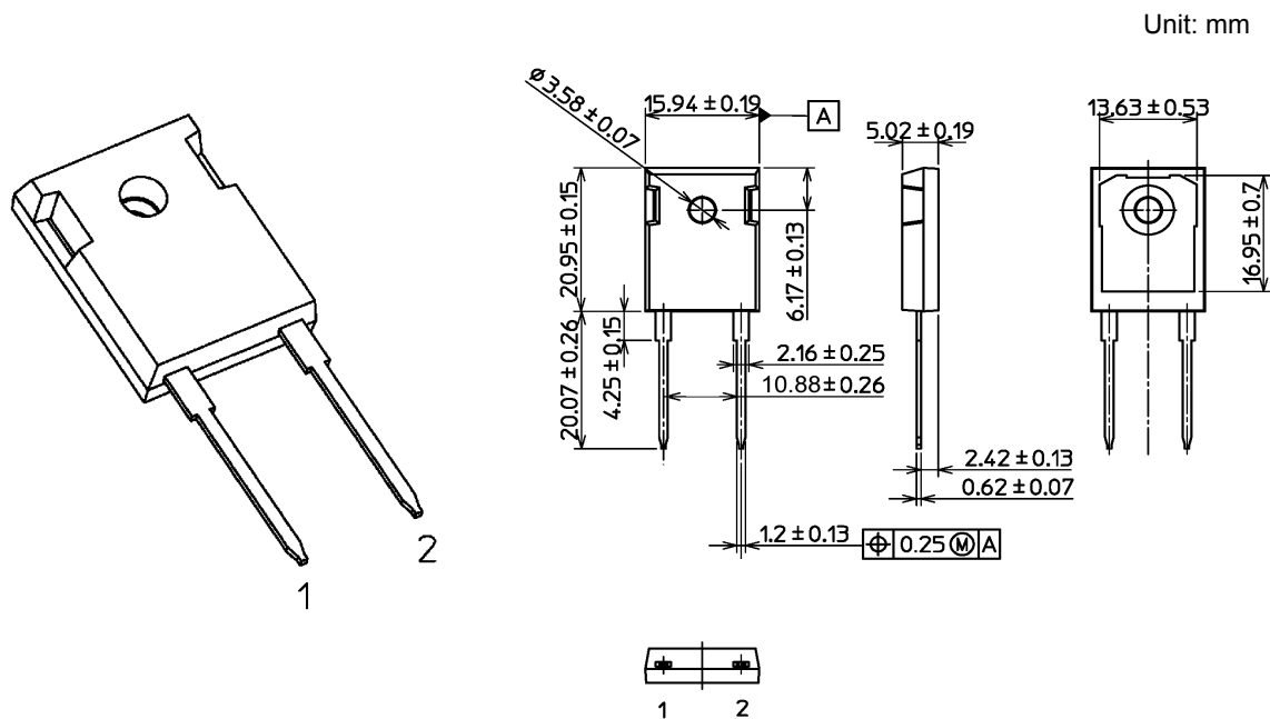
TO-247-2
