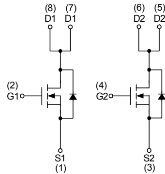
N-Channel MOSFET
