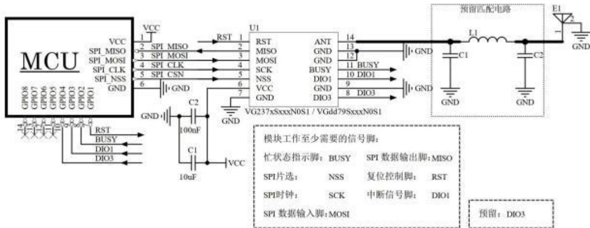
Figure 5-1 Programming development hardware connection
