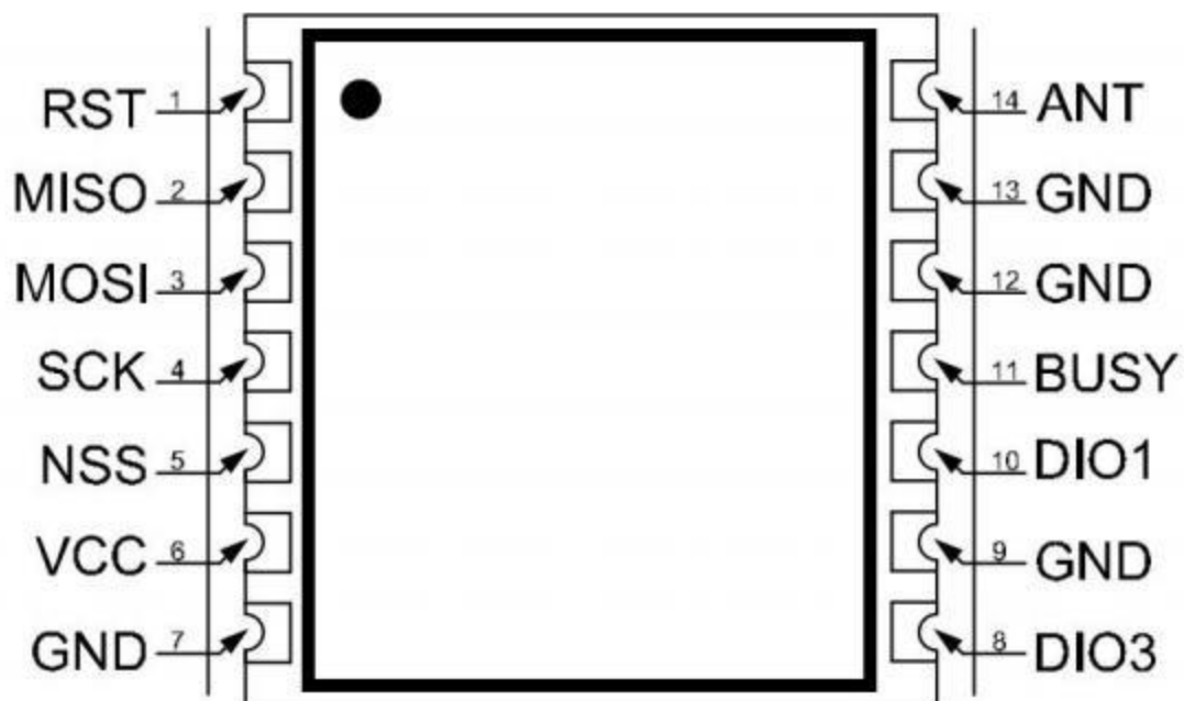
Figure 1-1 Top view
