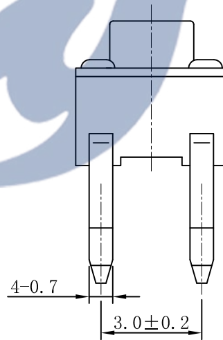
REFERENCE DRAWING
