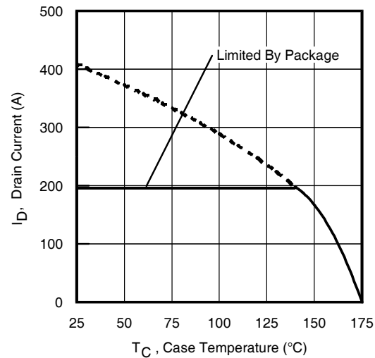
Fig 2. Maximum Drain Current vs. Case Temperature
