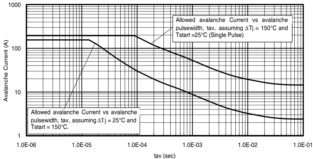
Fig 15. Typical Avalanche Current vs. Pulsewidth
