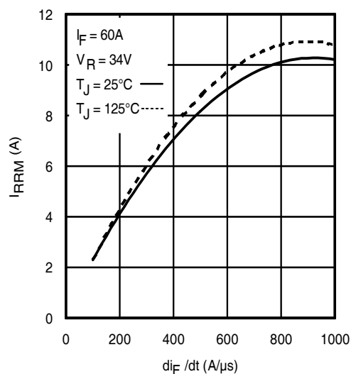
Fig 18. - Typical Recovery Current vs. di_F/dt
