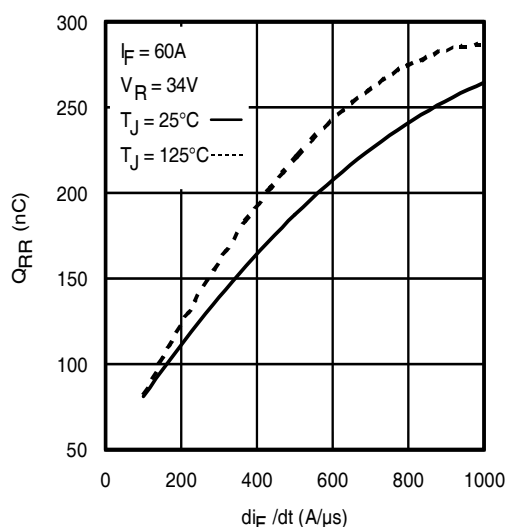
Fig 20. - Typical Stored Charge vs. di_F/dt
