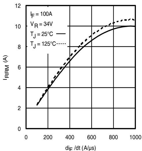
Fig 19. - Typical Recovery Current vs. di_F/dt
