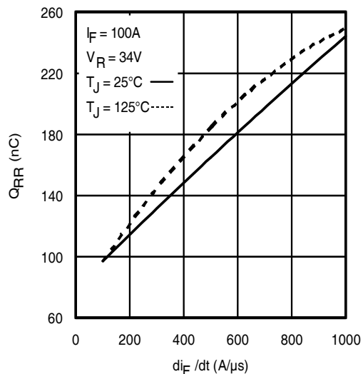
Fig 21. - Typical Stored Charge vs. di_F/dt
