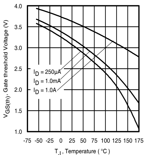
Fig 17. Threshold Voltage vs. Temperature
