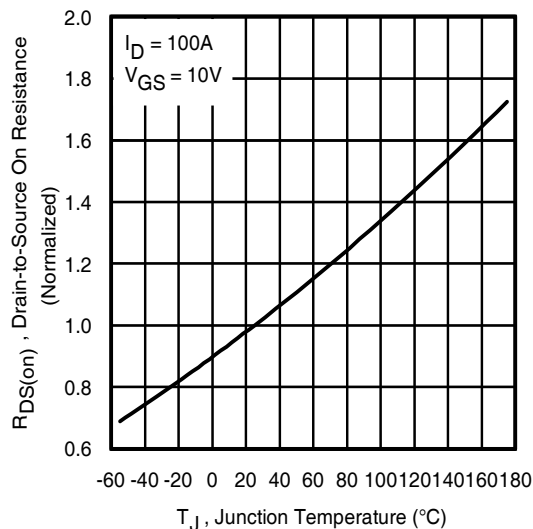
Fig 6. Normalized On-Resistance vs. Temperature
