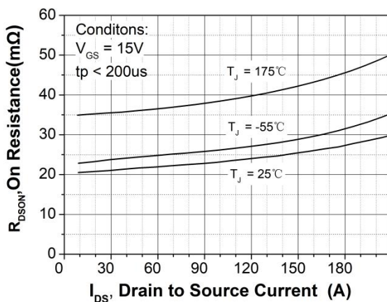
Figure 5. On-resistance vs. drain current for various temperatures
