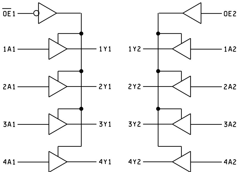
FIGURE 3. Logic diagram.
