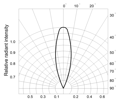
Fig.6 Radiation diagram
