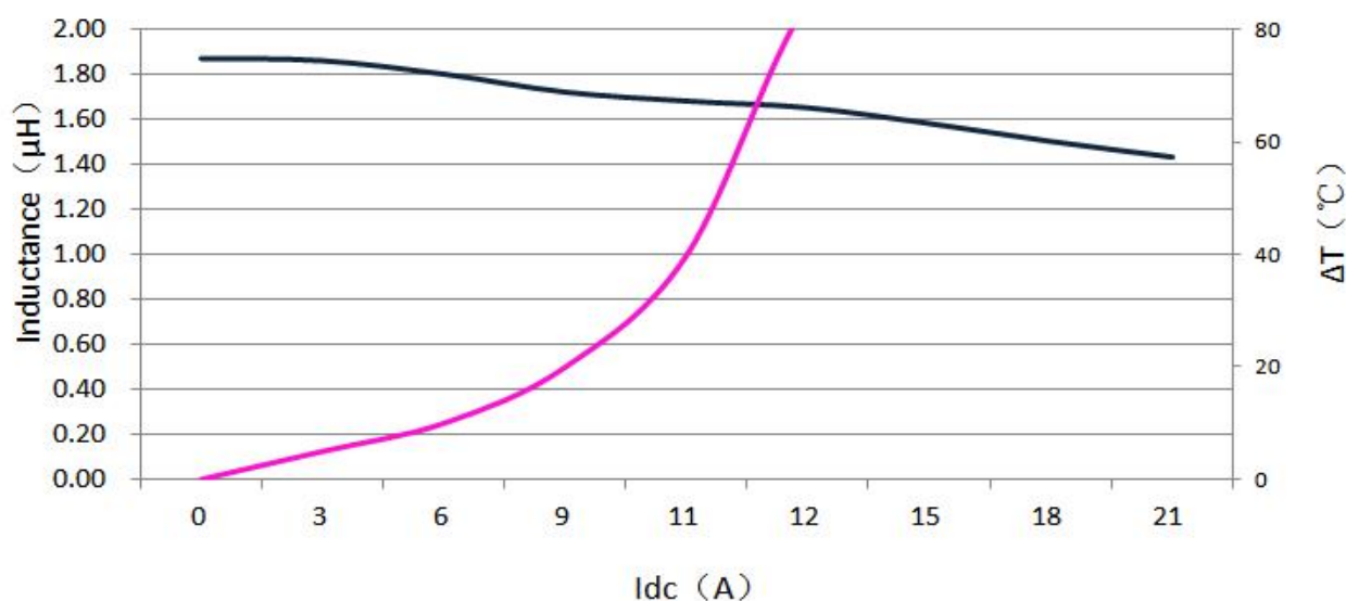
DC Current Curve
