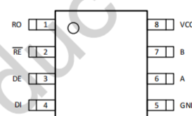
SOP-8
