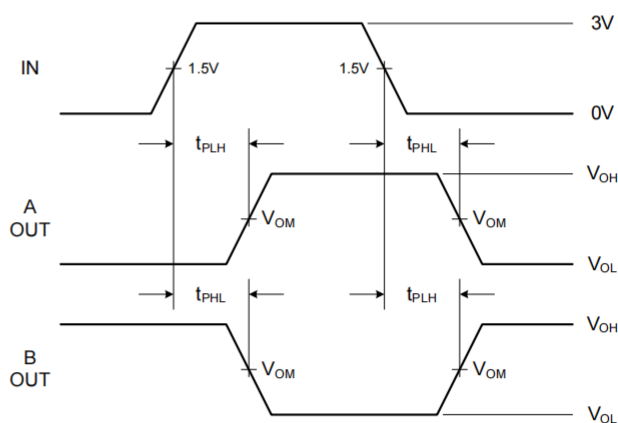
Fig. 4. Driver Propagation Delay
