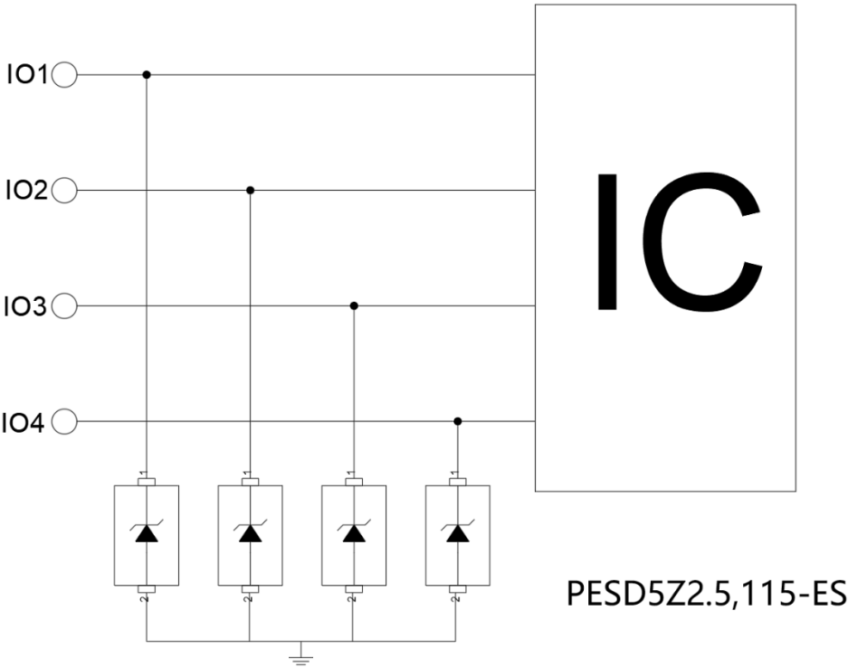
Pic-3 Typical Internet 1G Interface Application
