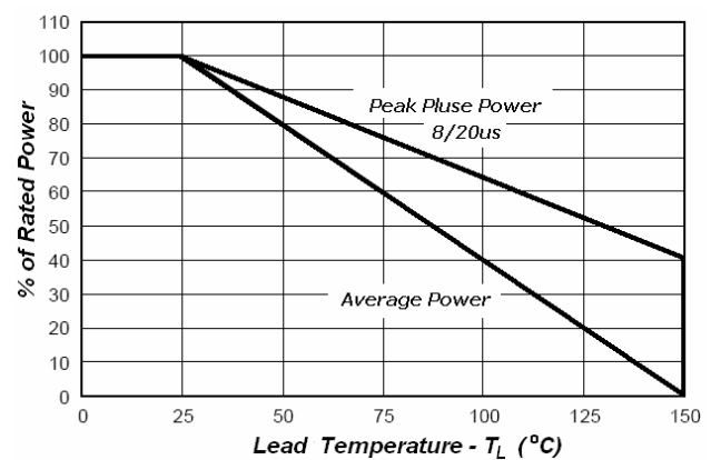
Fig 2. Power Derating
