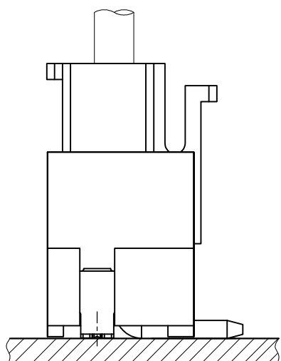
Assembly Layout
