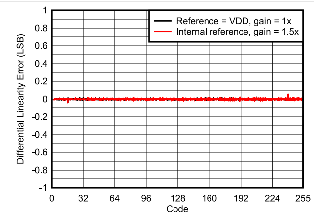
Figure 6-2. Differential Linearity Error vs Digital Input Code
