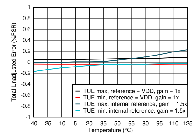
Figure 6-6. Total Unadjusted Error vs Temperature
