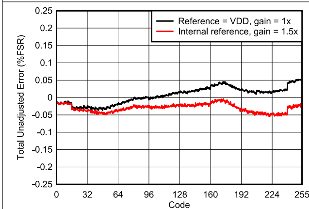
Figure 6-3. Total Unadjusted Error vs Digital Input Code
