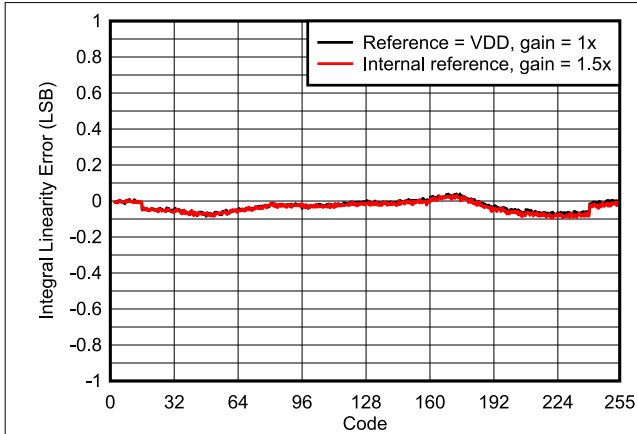
Figure 6-1. Integral Linearity Error vs Digital Input Code
