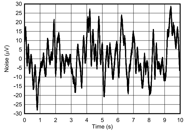
Figure 6-46. Digipot Output Noise: 0.1 Hz to 10 Hz
