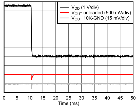
Figure 6-40. Power-off Glitch
