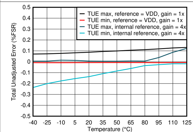
Figure 6-16. Total Unadjusted Error vs Temperature
