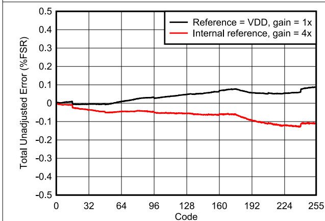
Figure 6-13. Total Unadjusted Error vs Digital Input Code
