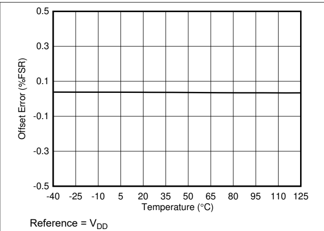
Figure 6-18. Offset Error vs Temperature
