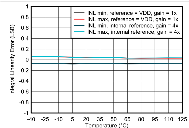
Figure 6-14. Integral Linearity Error vs Temperature
