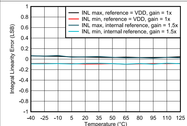
Figure 6-4. Integral Linearity Error vs Temperature
