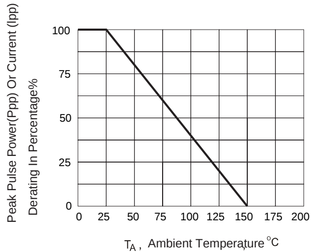
Fig.1 Derating Curve
