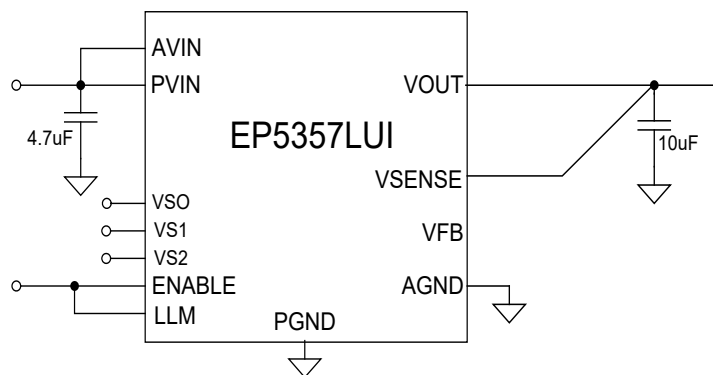
Figure 2: Typical Application Schematic
