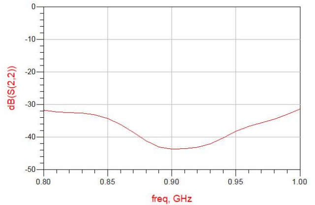
Figure 6. MHC0900M10 Return Loss (S22)
