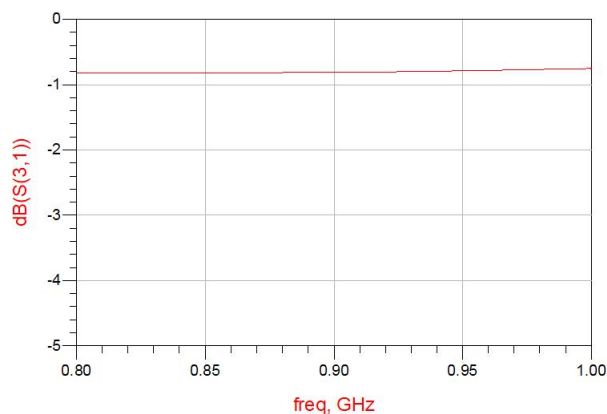
Figure 4. MHC0900M10 Transmission
