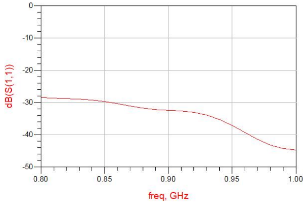
Figure 5. MHC0900M10 Return Loss (S11)
