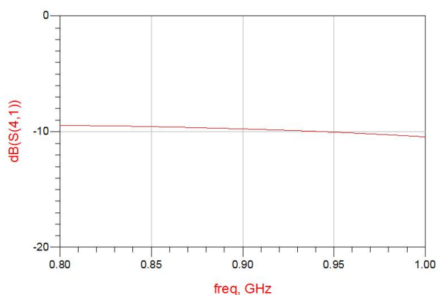
Figure 3. MHC0900M10 Coupling
