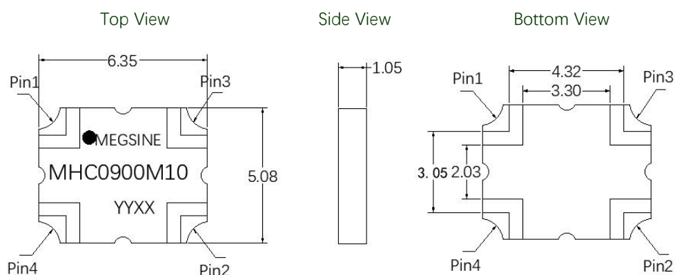
Figure 2. MHC0900M10 Outline Drawing
