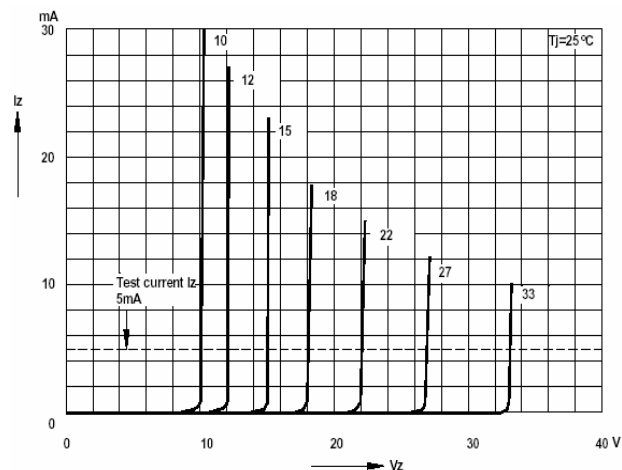
Breakdown characteristics at T_J = \text{constant} (pulsed)
