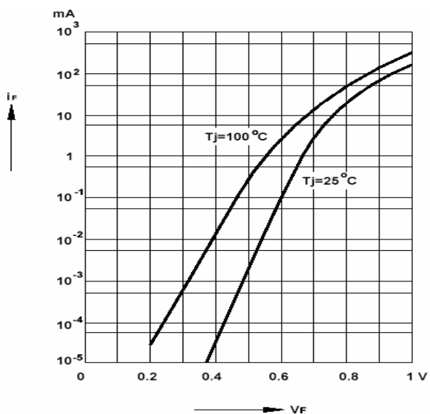
Forward characteristics
