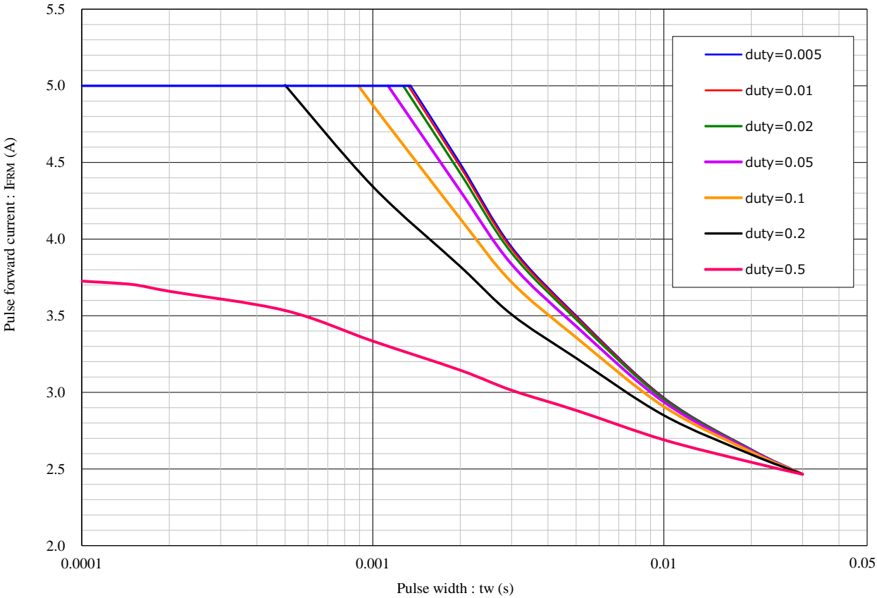
Maximum ratings of pulse forward current Condition : T_s = 85^\circ C
