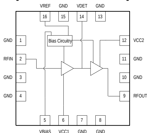
Figure 2. GSM0924 Function Block Diagram
