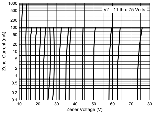
Fig. H- Typical Zener Breakdown Characteristics
