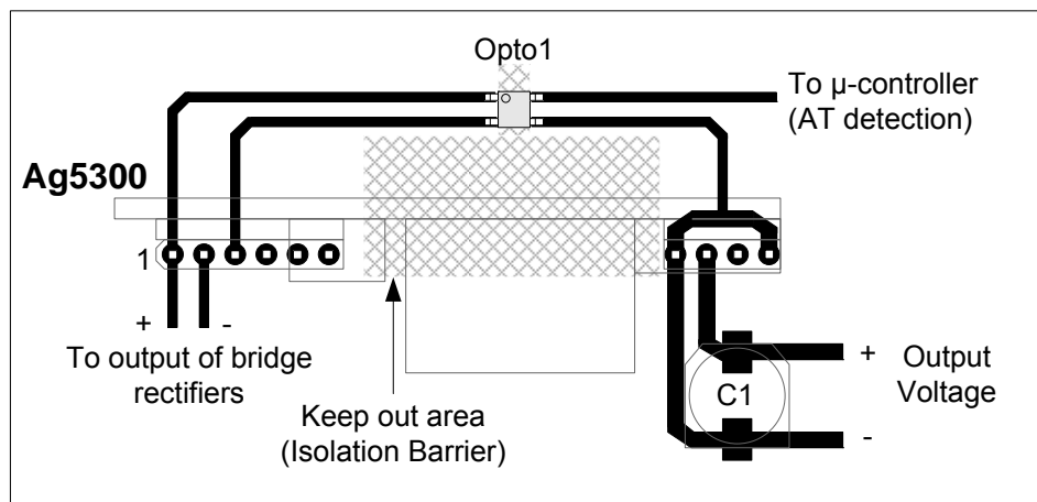
Figure 8: Layout Consideration
