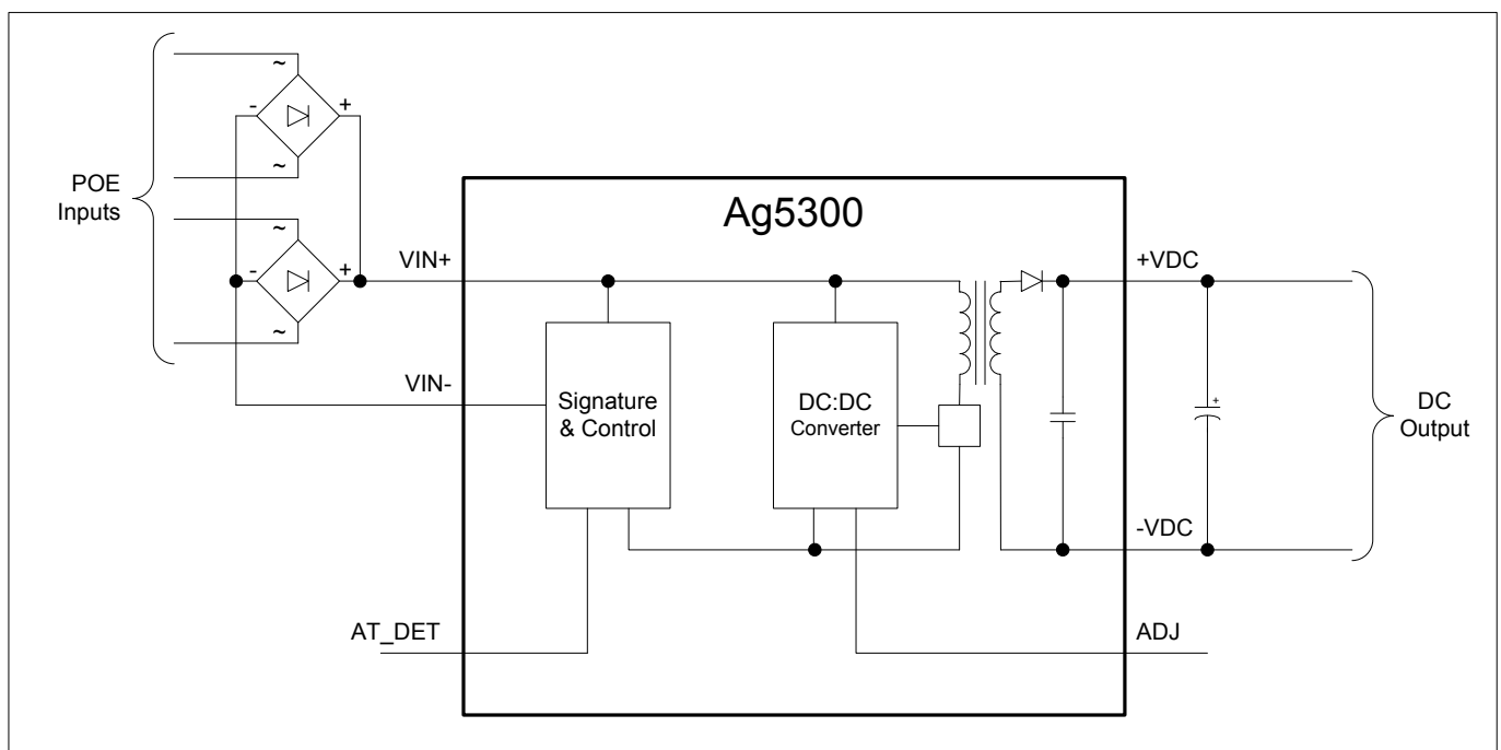
Figure 1: Block Diagram
