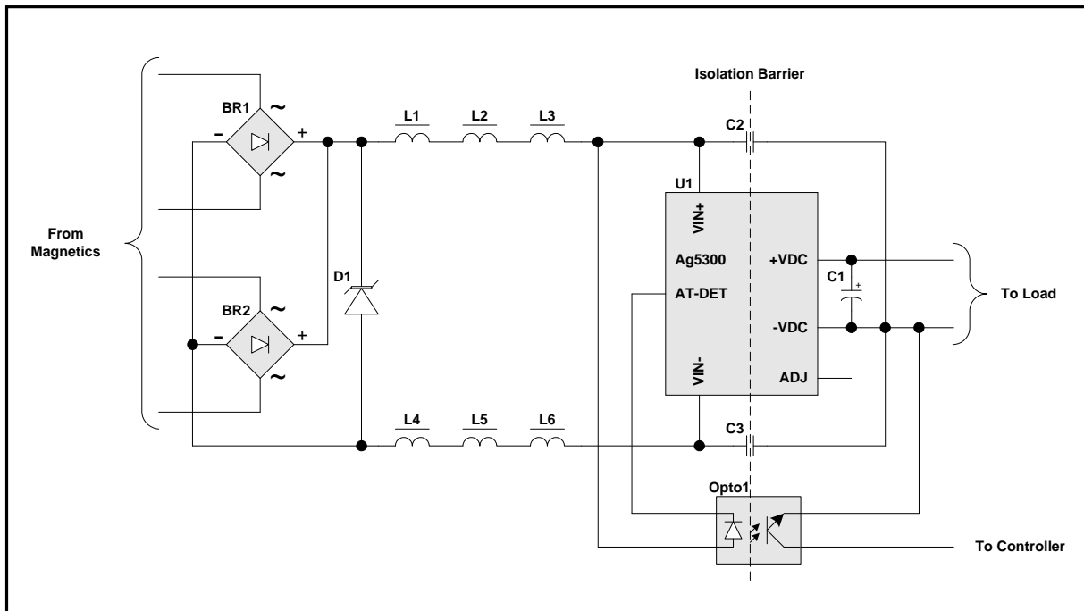
Figure 12: EMC Filtering
