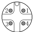
Pin Assignments Front View
