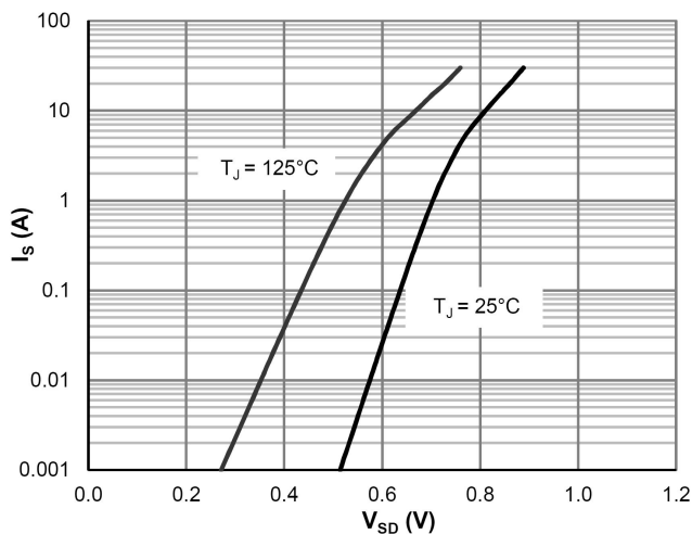
Body-Diode Characteristics
