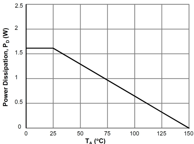
Power De-rating
