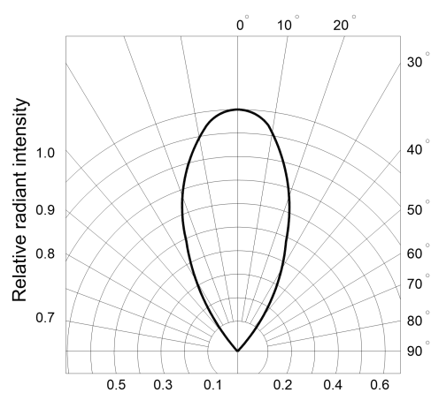
Fig.6 Radiation diagram
