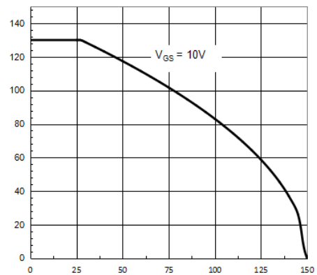
Figure 4. Drain Current
