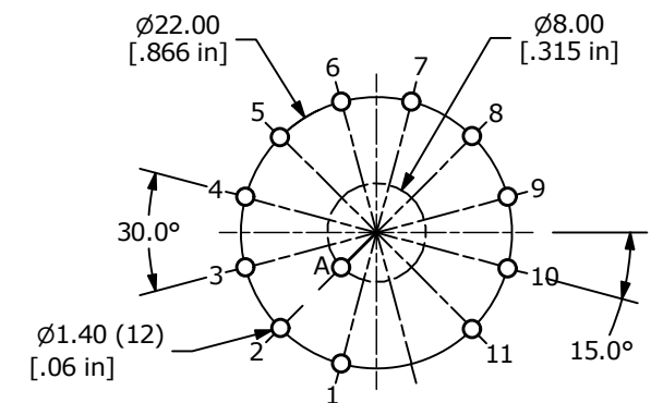
P.C.B MOUNTING LAYOUT
