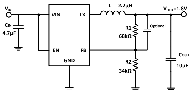
Figure 1. Basic Application Circuits
