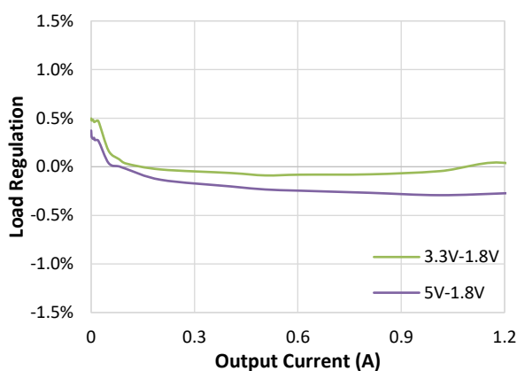
Load Regulation
