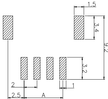
PCB.焊接图 PCB. WELDING DRAWING
