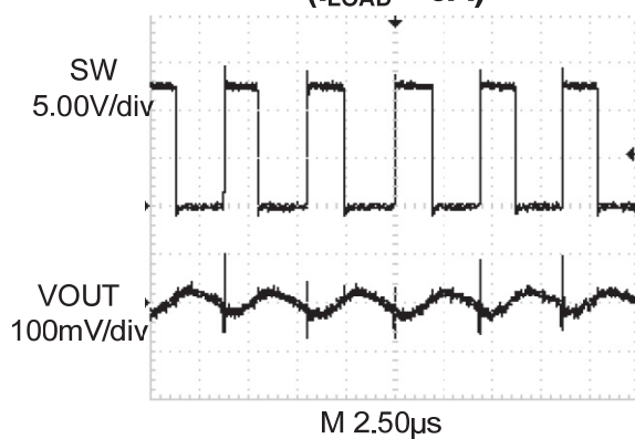
SW and Output Voltage ( I_{LOAD} = 0\text{A} )
