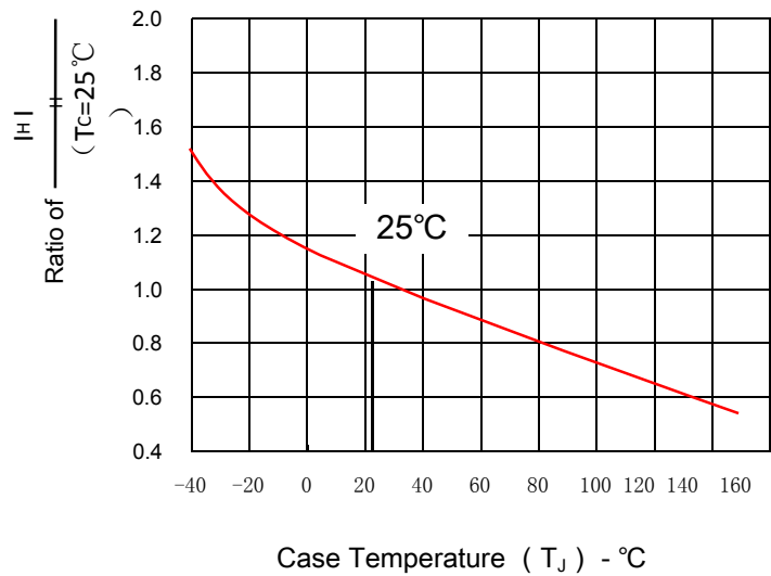
Figure 4. Normalized DC Holding Current versus Case Temperature
