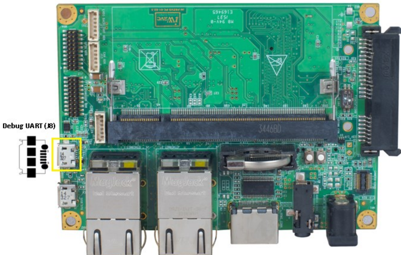
Figure 3: Debug UART
