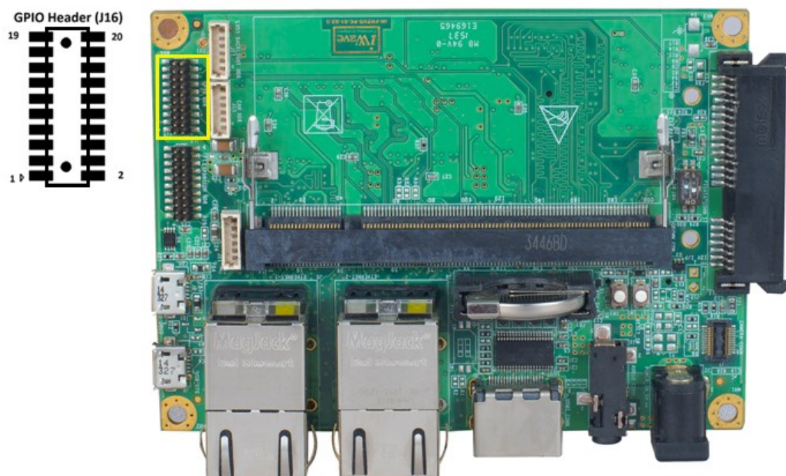
Figure 20: GPIO Header
