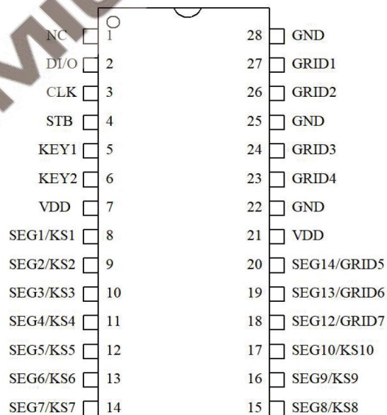
HTM16 67 28SOP
