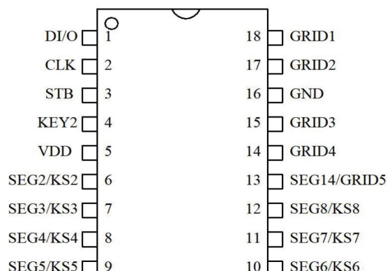
HTM1630 18DIP
