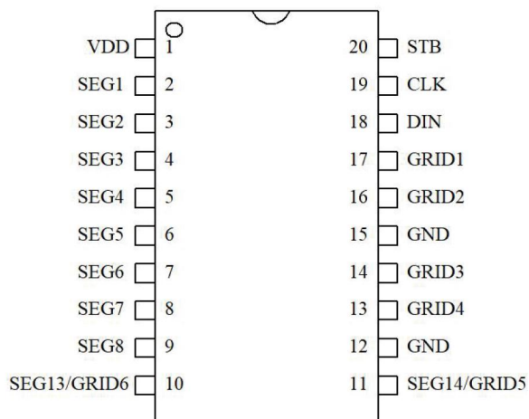
HTM16 20 20SOP
