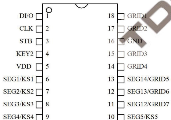
HTM16 18 18SOP
