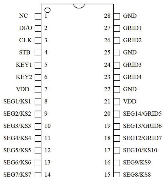
HTM1628 28SOP/SSOP
