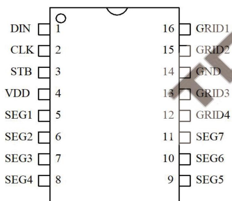
HTM16 16 16SOP
