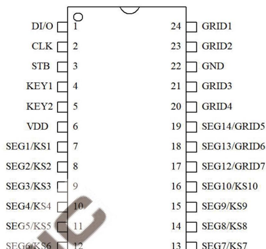
HTM1668 24SOP/SSOP
